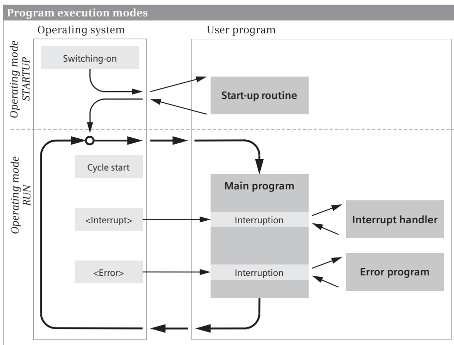
Fig. 1.2 Execution of the user program in a SIMATIC controller
