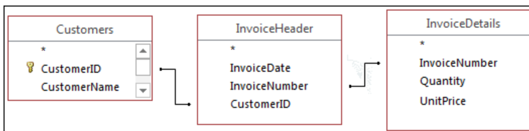
Figure 1-2: Databases use relationships to store data in unique tables and simply relate these tables to each other.
